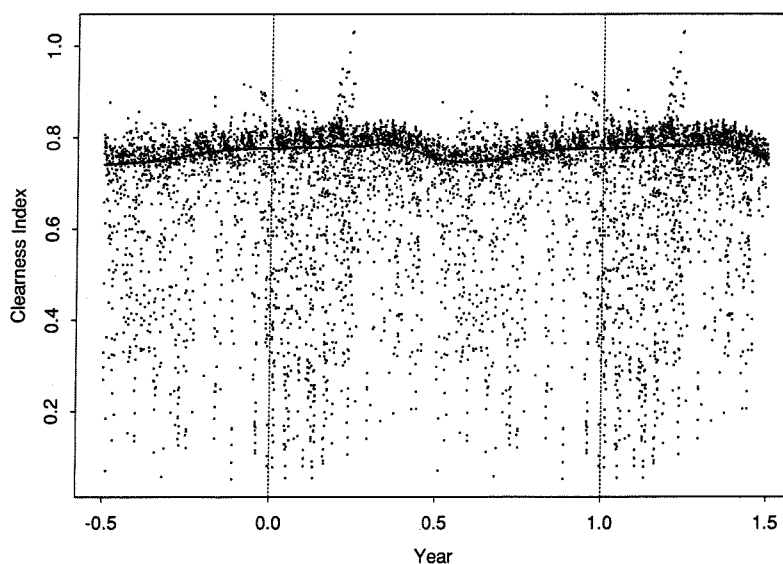
Fig. 5. Overplot of all background clearness index data for Las Cruces, NM, before 1991 June onto a single year with zero (0) 1 January and one (1) 31 December of each year. Smoothed line is robust estimate with approximately monthly time resolution.
