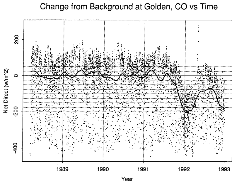
Fig. 10. Time series plot of net direct irradiance with background of Fig. 9 removed according to time of year that data were measured for Golden, CO. Smoothed line is robust estimate with approximately monthly time resolution.
