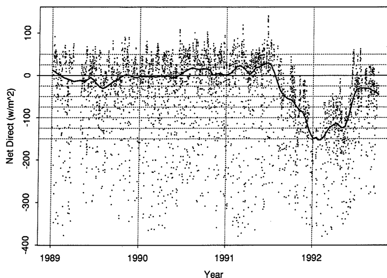
Fig. 4. Time series plot of Fig. 2 with background from Fig. 3 removed according to the time of year the data were measured. Smoothed line is robust estimate of net change with approximately monthly time resolution.
