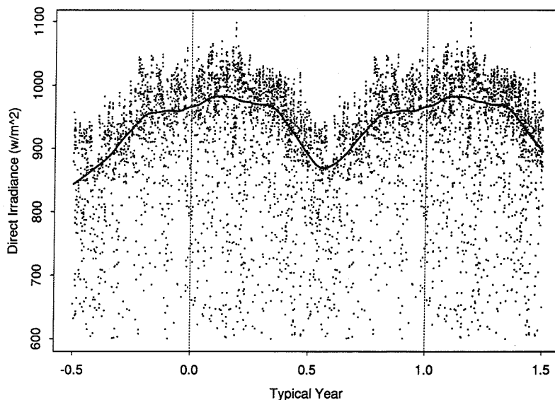
Fig. 3. Overplot of all background data from Fig. 2 before 1991 June onto a single year with zero (0) 1 January and one (1) 31 December of each year. Smoothed line is robust estimate with approximately monthly time resolution.
