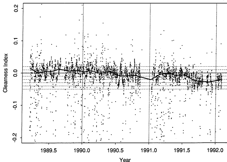
Fig. 12. Same as Fig. 6 except 10-minute data within one hour of local noon for Kramer Junction, CA (SEGS site) and background data of Fig. 11 subtracted.
