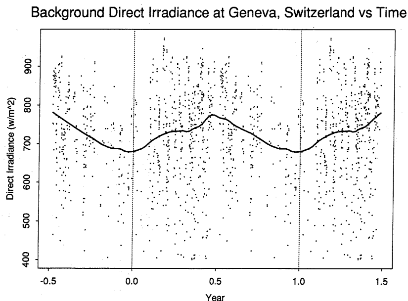
Fig. 7. Same as Fig. 3 except for Geneva, Switzerland, with 400 \text{ W/m}^2 threshold. Geneva background contains one less year of data than Las Cruces.
