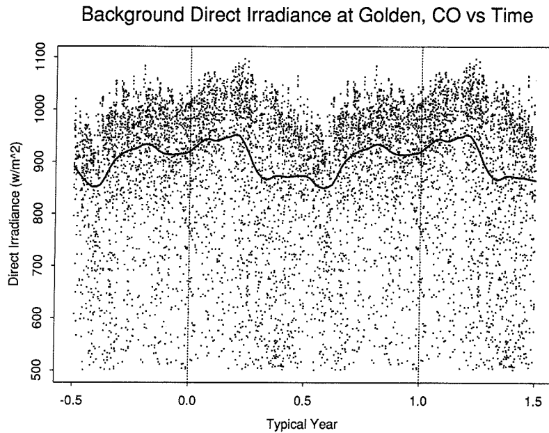
Fig. 9. Same as Figs. 3 and 7 except for Golden, CO, with 500 \text{ W/m}^2 threshold and hourly averages within three hours of local noon.
