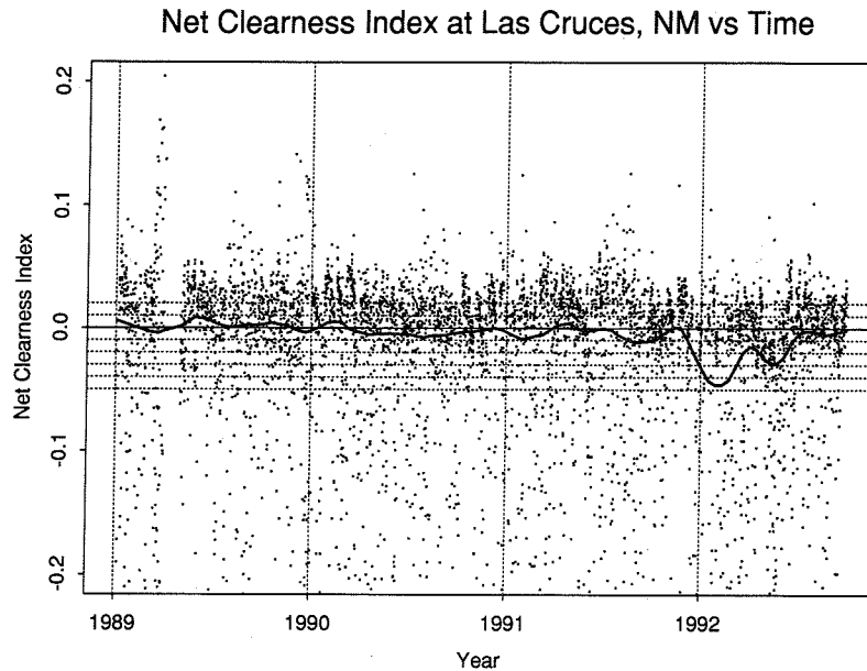
Fig. 6. Time series plot of net clearness for Las Cruces, NM, obtained by subtracting background clearness of Fig. 5 from entire time series of clearness. Smoothed line is robust estimate with approximately monthly time resolution.
