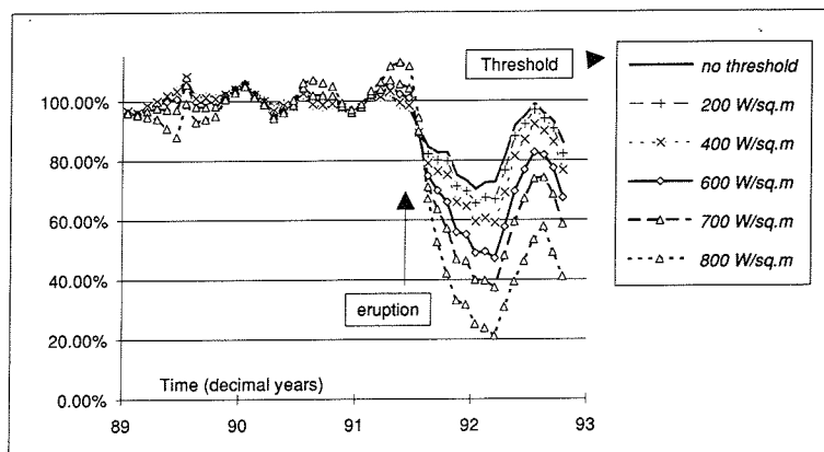
Fig. 13. Plot of direct solar energy loss relative to background and its dependence on operating thresholds for a SEGS-like facility in Las Cruces.
