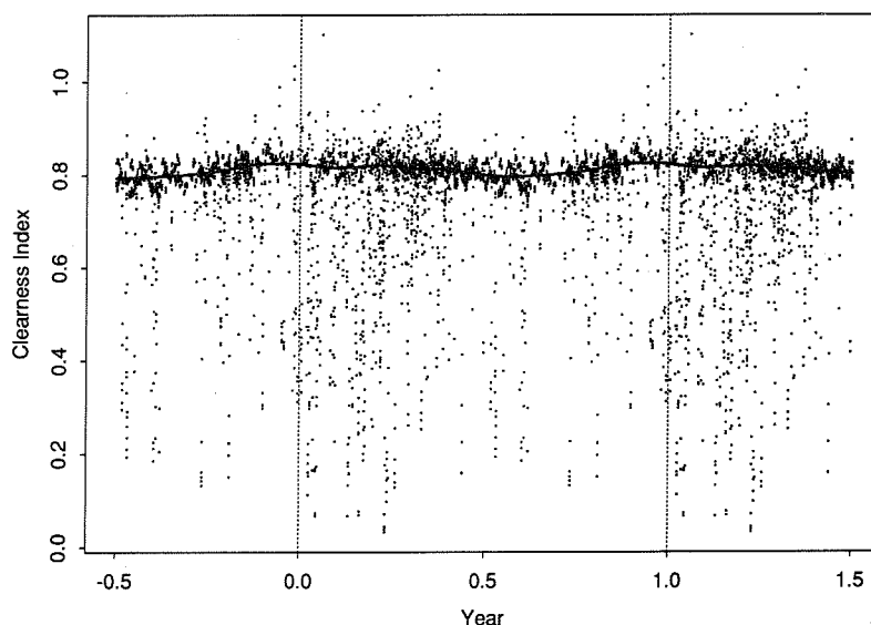
Fig. 11. Same as Fig. 5 except 10-min data within one hour of local noon for Kramer Junction, CA (SEGS site).
