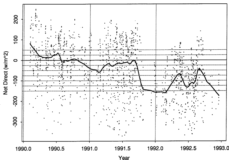
Fig. 8. Time series plot of net direct irradiance with background of Fig. 7 removed according to time of year that data were measured for Geneva, Switzerland. Smoothed line is robust estimate with approximately monthly time resolution.
