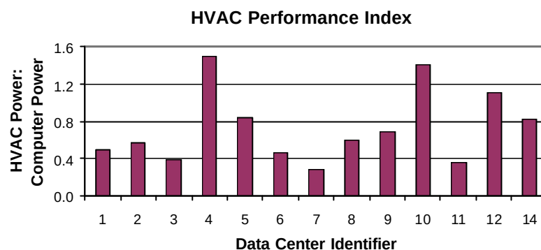
Figure 5. Relative data center HVAC system performance
