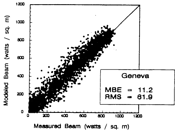
Figure 7 Modeled vs. measured direct irradiance using the 4-D algorithm.
