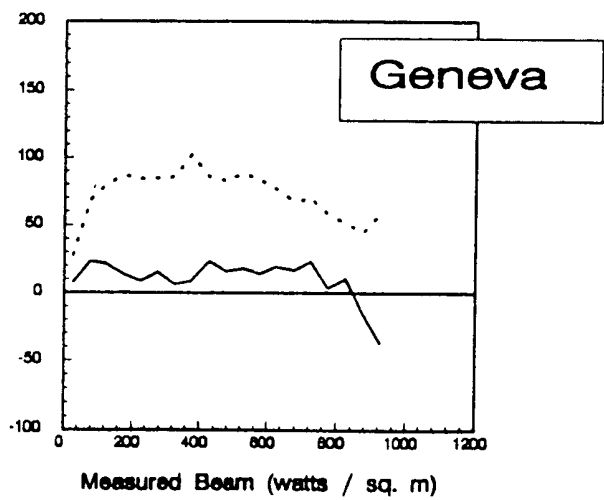
Figure 11 Model RMSE and MBE as a function of incoming direct irradiance for the 4-D algorithm.
