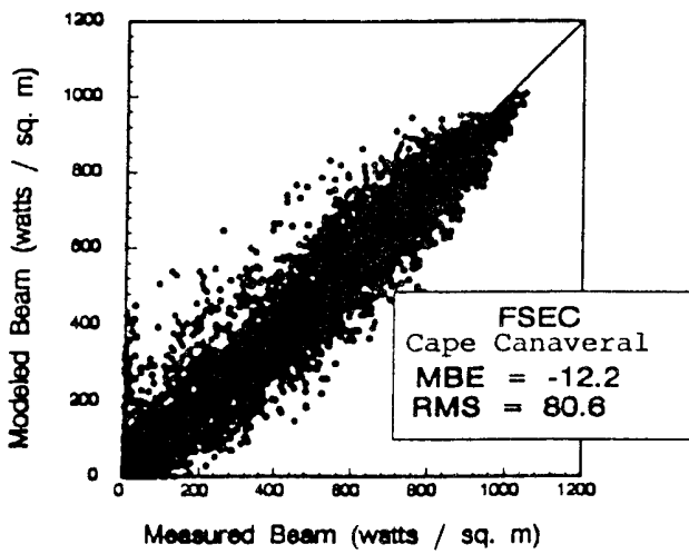
Figure 7 Modeled vs. measured direct irradiance using the 4-D algorithm.
