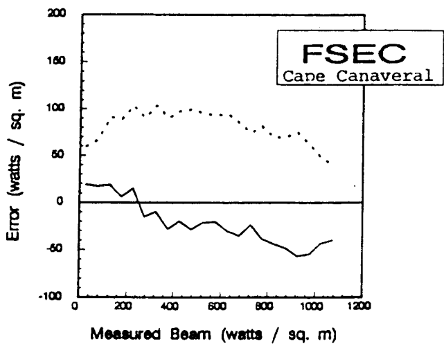
Figure 11 Model RMSE and MBE as a function of incoming direct irradiance for the 4-D algorithm.
